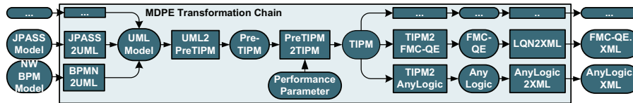
Figure 1: MDPE Transformation chain for interconnecting two or more Process Modelling Tools with two or more Performance Analysis Tools as Block Diagram ([KGT06])
