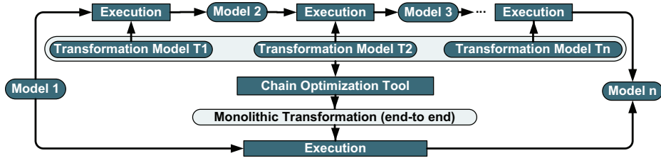
Figure 2: Transformation chain optimization overview as Block Diagram ([KGT06])
